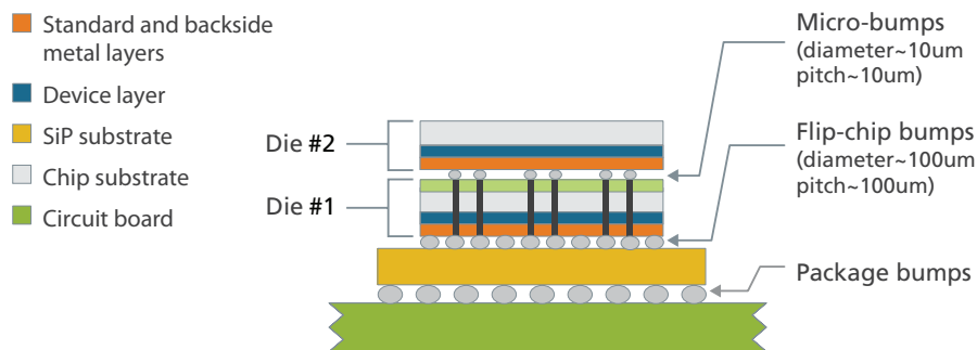
Figure 3: A simple 3D IC using TSVs
