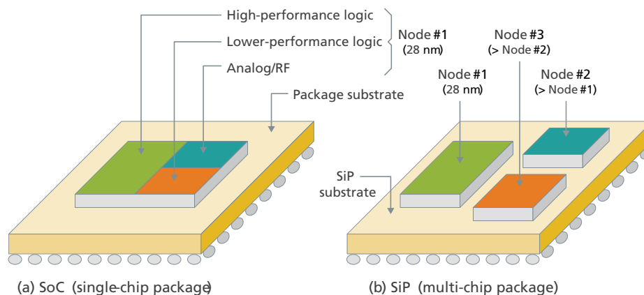
Figure 1: System-on-Chip (SoC) compared to System-in Package (SiP)
