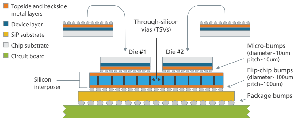
Figure 2: Adding a silicon interposer with TSVs (only two die are shown for simplicity)
